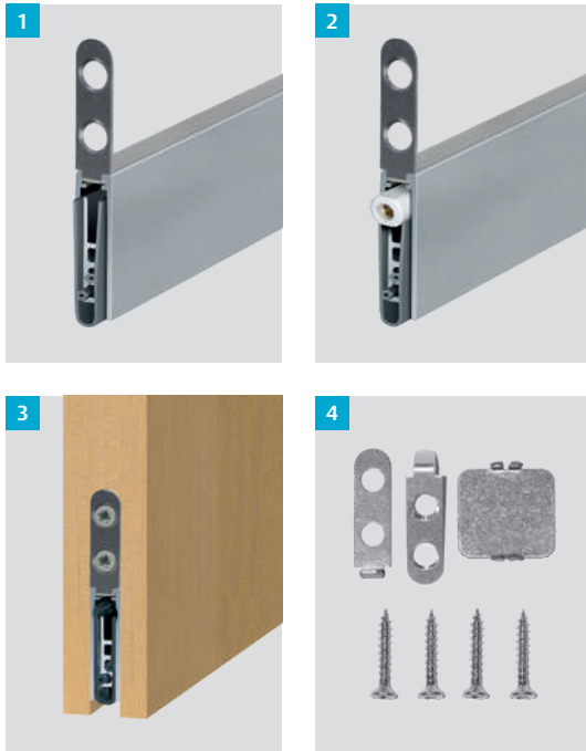
1. Profile Planet US with fastening brackets for wooden doors 2. Planet US with fastening brackets, release side 3. Planet US installed in especially narrow doors 4. Planet assembly set TW/US for wooden doors (standard)
