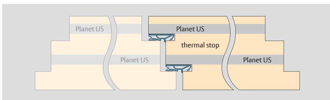
Example 4: doors with two sealing levels (thermal stop)
