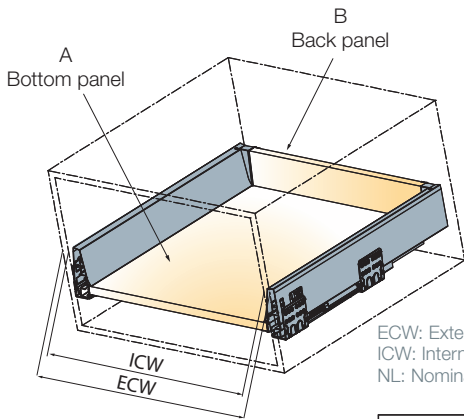
Cutting dimensions details
