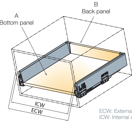
Cutting dimensions details
