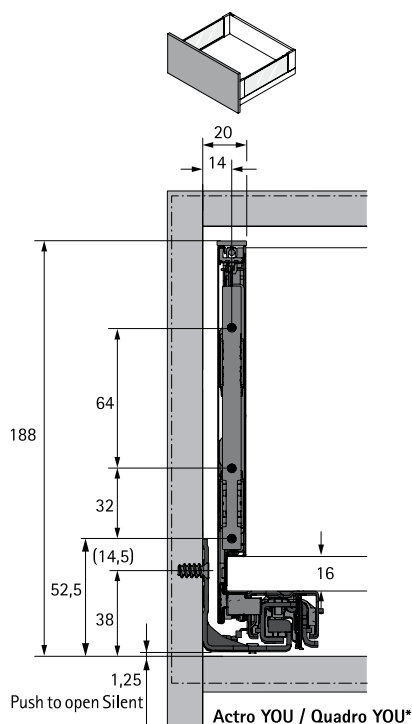
Actro YOU / Quadro YOU*
